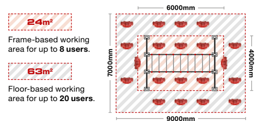
OHTS823 Octagon HTS 8 Leg 2x3 Beam
